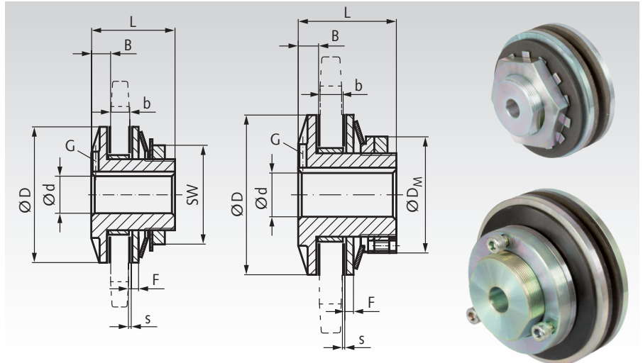
Up to No. 612 040 00 with hexagonal nut
